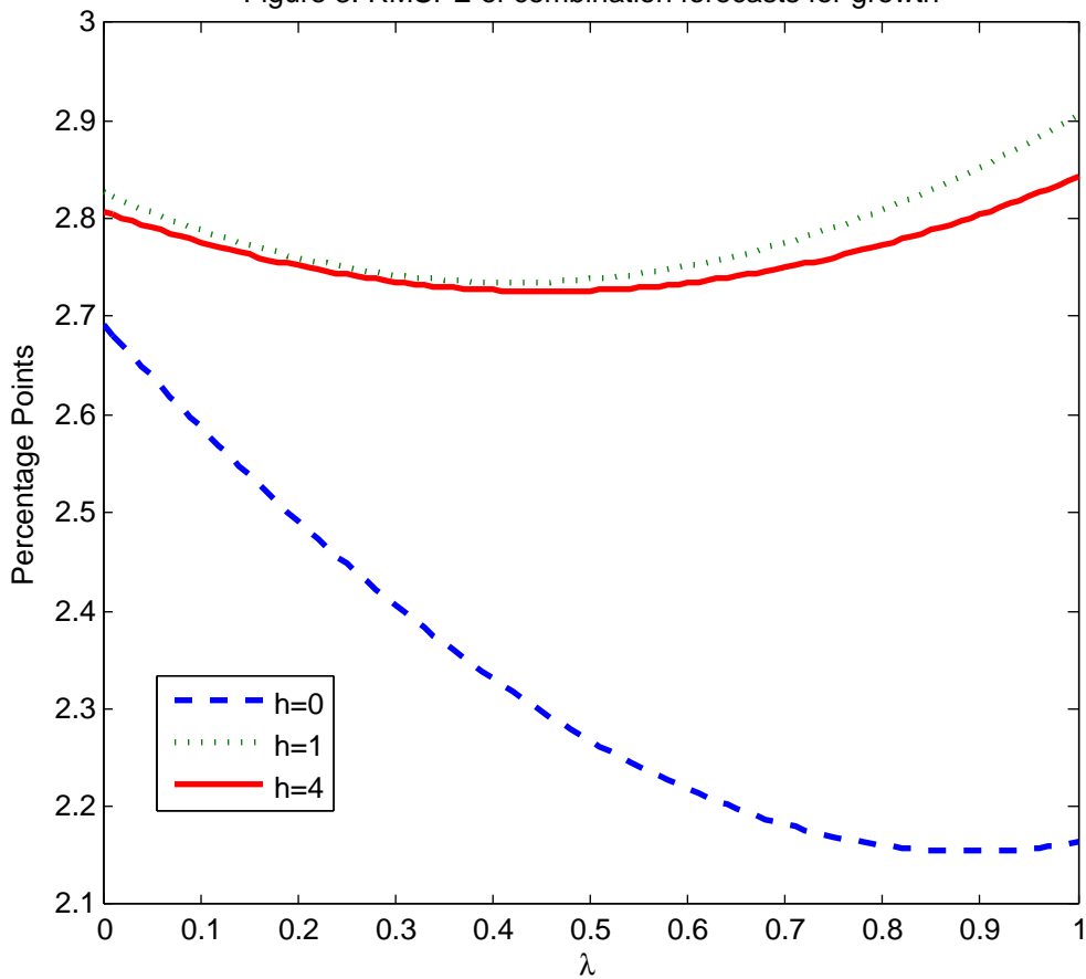
Figure 3: RMSPE of combination forecasts for growth
