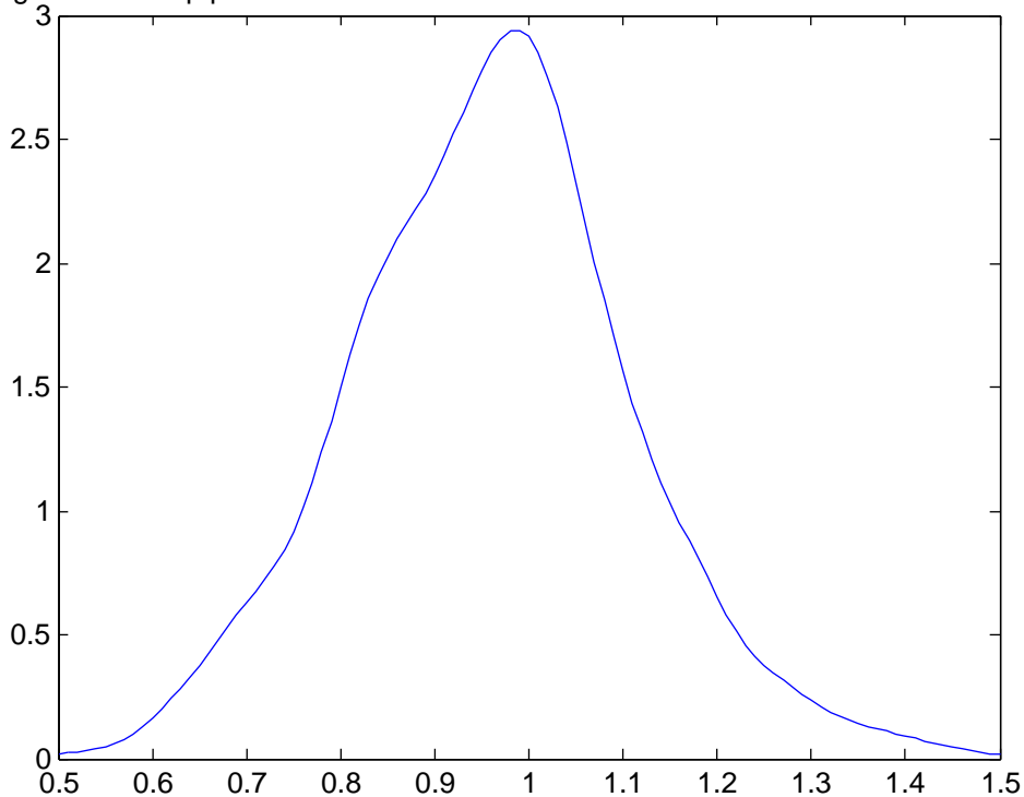
Fig. 1: Bootstrap pdf for the ratio of GB to RW RMSEs in Atkeson–Ohanian sample
