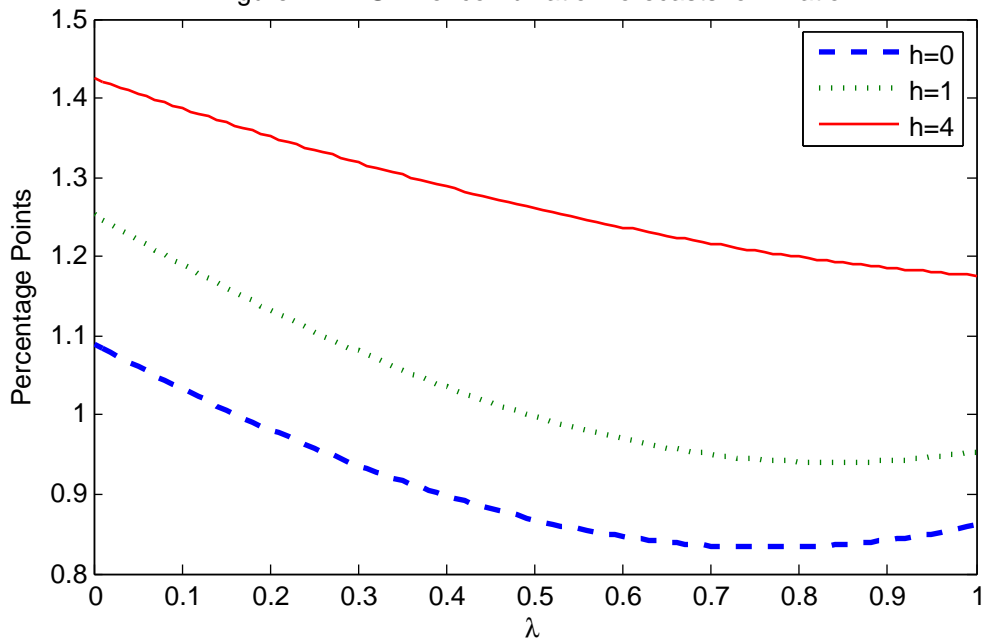
Figure 2: RMSPE of combination forecasts for inflation
